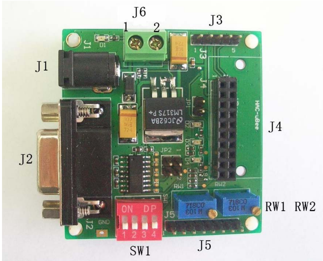
Picture 4 HAC-UBee TEST BOARD
