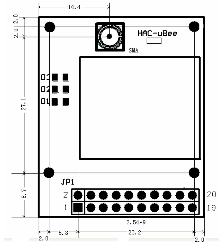
Picture 3 Structure dimension of HAC-UBee V1.3
