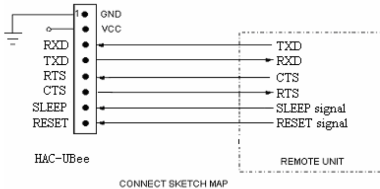
Picture 1: Connection sketch between HAC-UBee and terminal equipment
